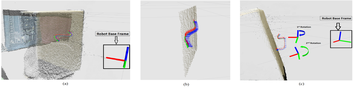
Fig. 3: Visualization of experimental results with the rectangular box. The blue arrows represent the normal vector to the surface, whereas the green and red arrows represent the tangential axes to the surface. (a) The rectangular box is stationary and the reference path is fitted on its surface. The orientation is calculated w.r.t the robot base frame. (b) A zoomed and segmented version of the box's front side providing a more clear aspect of the path fitted on the surface. (c) The box is rotated initially w.r.t. the z (blue) axis and then w.r.t. the y (green) axis and the calculated path adapts to this motion.
