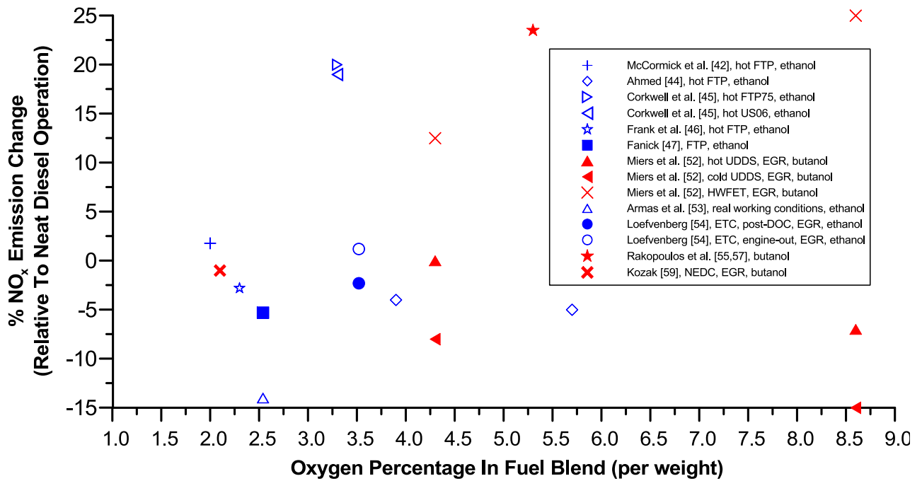
Fig. 11. Collective NO x emissions change from ethanol and n-butanol/diesel fuel blends combustion during transient schedules (for those studies where no relevant information was available, it was assumed that the oxygen content of the reference diesel fuel was zero; for Rakopoulos et al. [55,57], average-cumulative NO (and not NO x ) values are taken from three accelerations and one hot starting).
