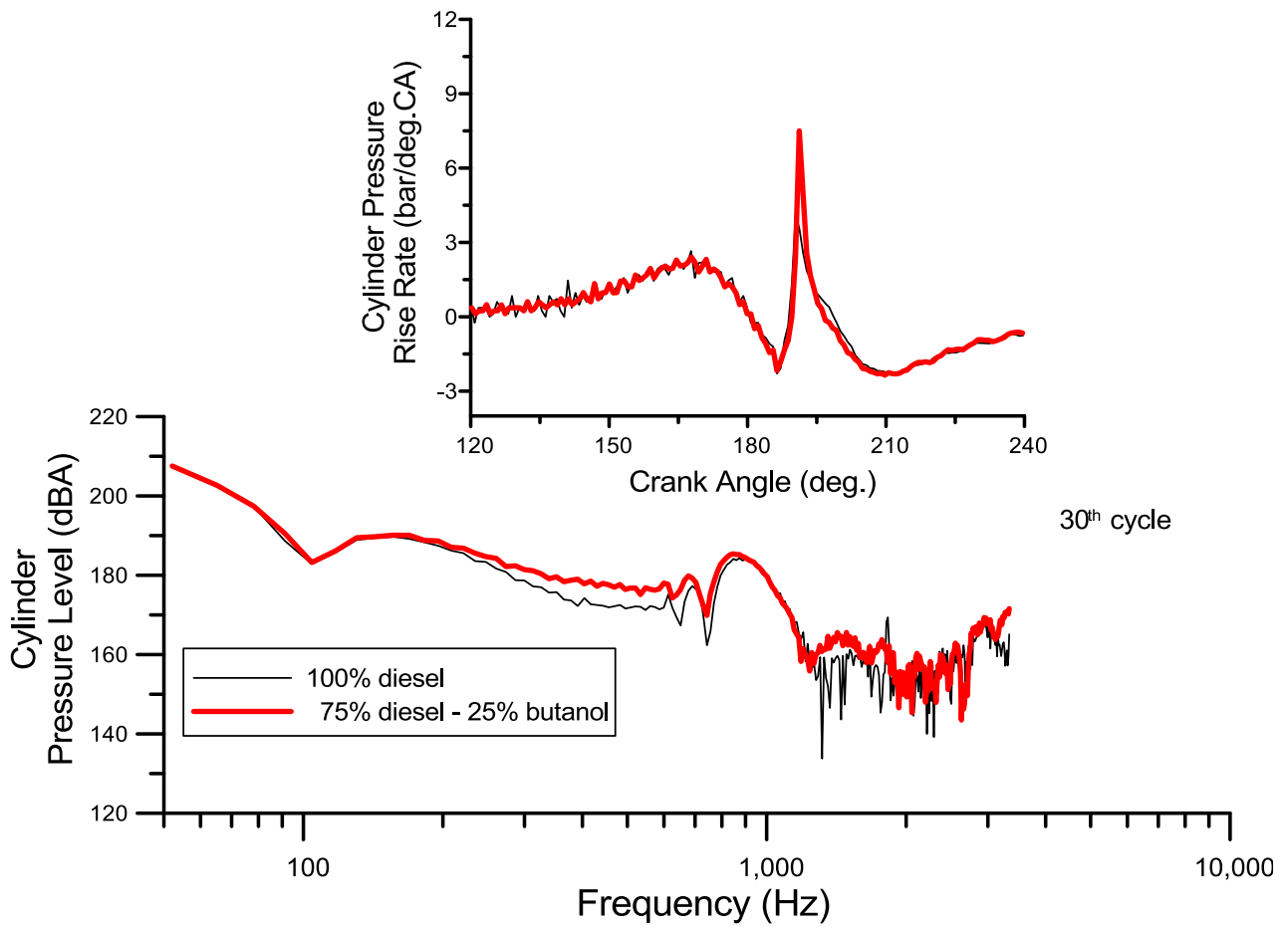
Fig. 16. Cylinder pressure rise rate and sound level during the 30 th cycle of the acceleration test of Fig. 14 [62].
