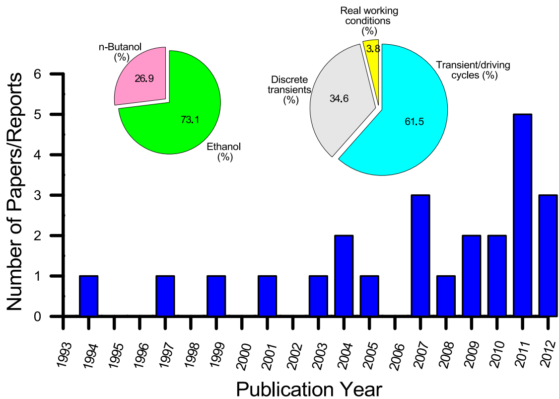
Fig. 2. Quantification of published papers/reports on transient diesel engine emissions with ethanol or n-butanol/diesel blends in a chronological order (main figure) up to 2012, based on the alcohol used (upper left), or the transient schedule tested (upper right)
