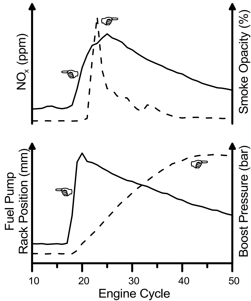
Fig. 1. Qualitative fueling vs. air-supply (boost pressure) response, highlighting the turbocharger lag and its inter-relation with smoke opacity and NO x emission spikes, typical at the onset of each acceleration or load-increase event.
