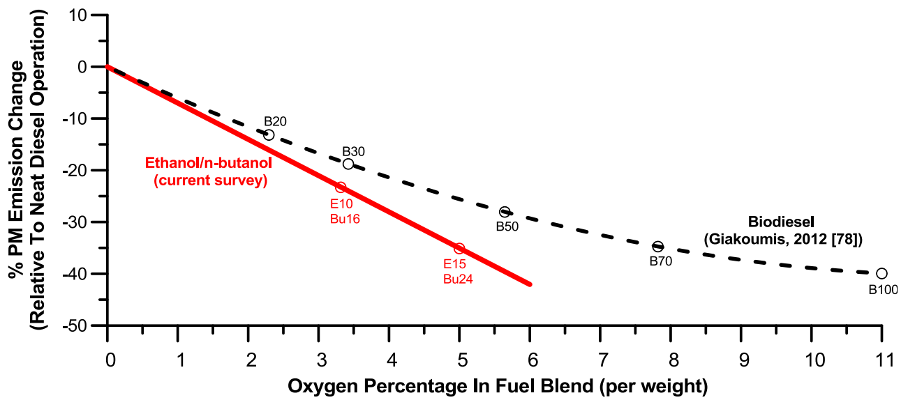
Fig. 12. Statistical results of ethanol or n-butanol/diesel blends PM emission benefit over neat diesel operation (solid red line) in comparison with biodiesel blends (discontinuous black line) during transient cycles.
