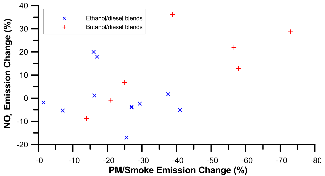
Fig. 14. PM/ \text{NO}_x trade-off from ethanol and n-butanol/diesel fuel blends combustion during transient schedules (smoke values instead of PM are used for those studies that did not measure PM)
