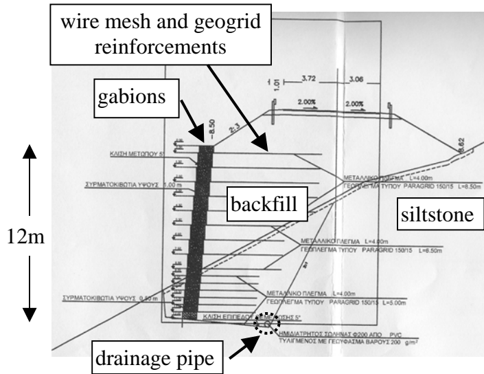
Figure 1. Cross section of reinforced wall and embankment considered in stability calculations.
