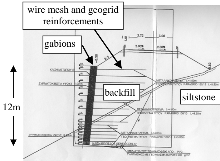
Figure 1. Cross section of reinforced wall and embankment considered in stability calculations.
