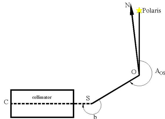
Figure 3: The elements for the determination of the collimator's axis astronomical azimuth
