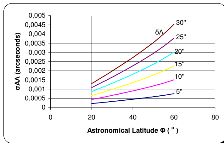
Figure 6: Diagram of the error \sigma_{A_\Lambda} relative to the estimation of the value of \Lambda ( \delta_\Lambda ) and the astronomical latitude of the observation place \Phi .
