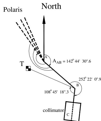
Figure 7: Formation arrangement measurements.
