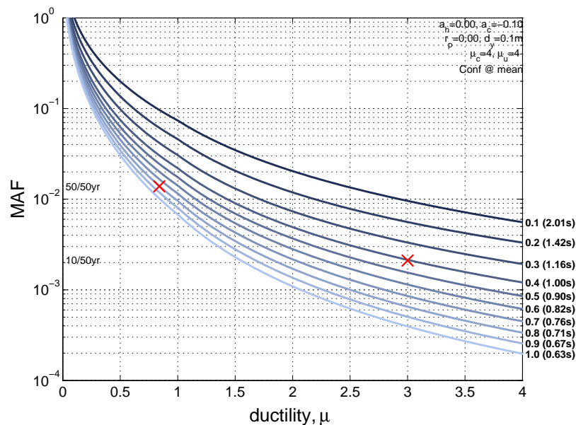
Fig. 5 YFS contours at C_y = 0.1, \dots, 1.0 for designing a 4-story steel frame at Van Nuys, CA. The red “x” symbols represent two performance objectives ( \mu = 0.84 , 3 at 50% and 10% in 50yrs exceedance rates, respectively). The first objective governs with C_y \approx 0.81 corresponding to a period of T \approx 0.71\text{s} .
