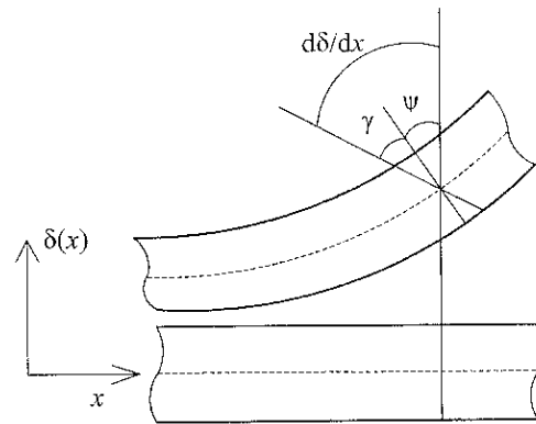
Fig. 3 Bending and shear rotation of a Timoshenko beam
