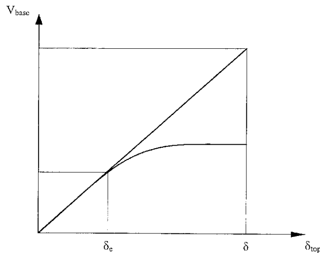
Fig. 1 Base shear top displacement curve of a frame
