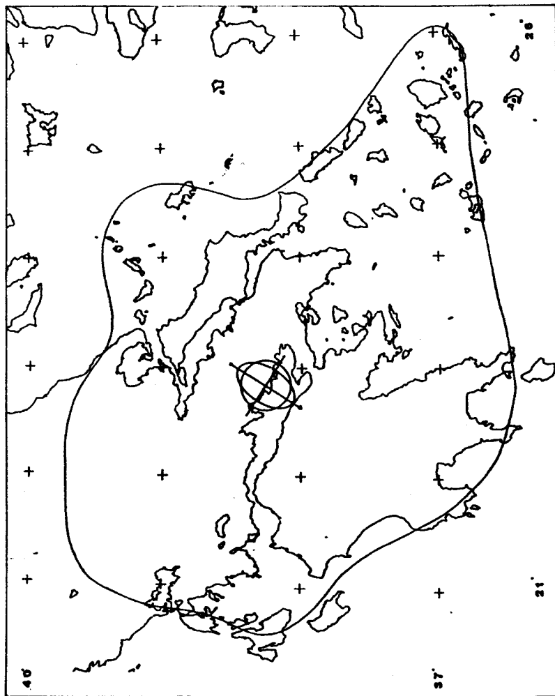
Fig. 3. Delineation of the area under investigation with the deformations expressed by a single tensor.
