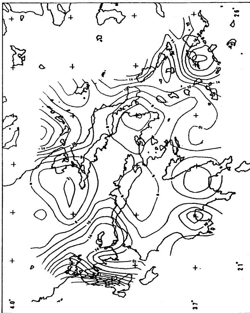
Fig. 7. The shear strain obtained by scanning in half degree step both in latitude and longitude.
