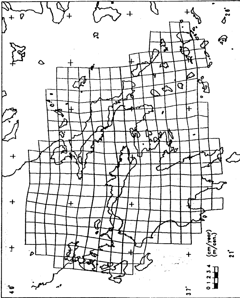
Fig. 5. The distorted grid 20 km x 20 km over a period of 1 My.
