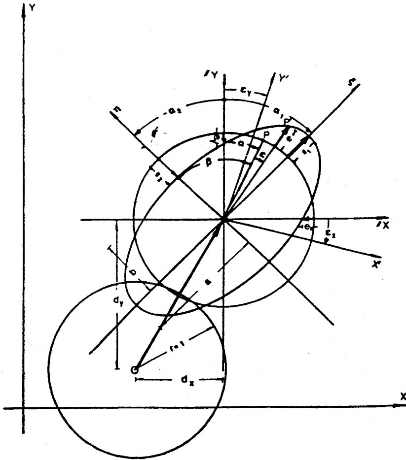
Fig. 1. The strain ellipse.
