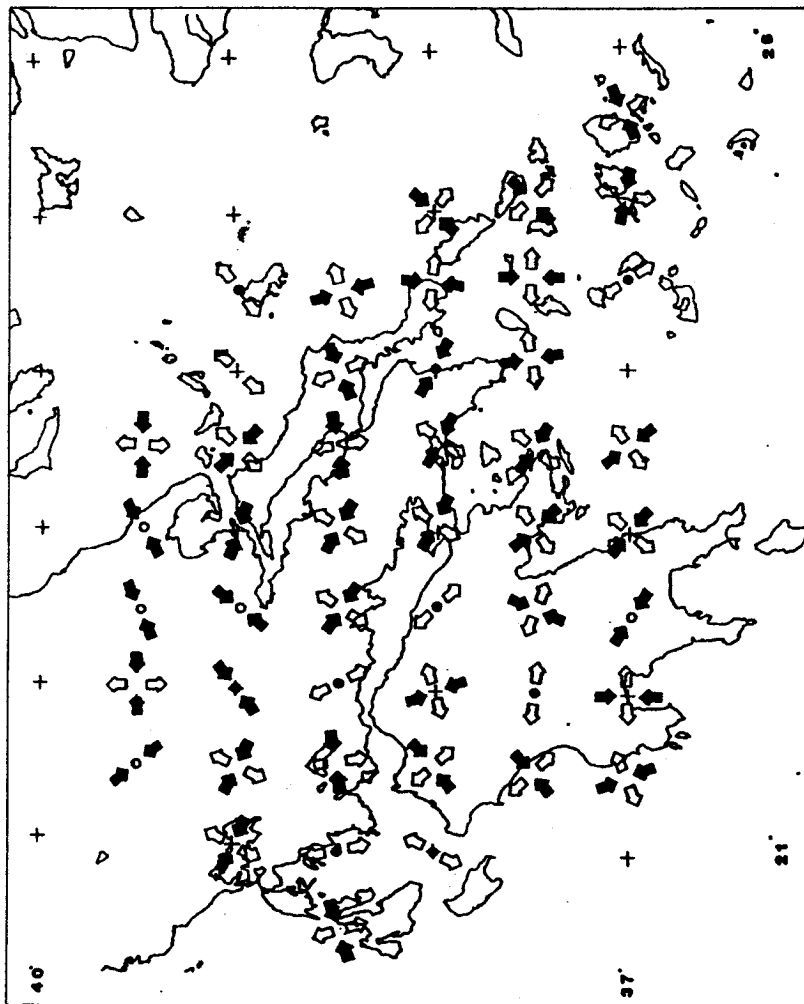
Fig. 8. The principal axes of strain obtained by scanning in half degree step both in latitude and longitude.
