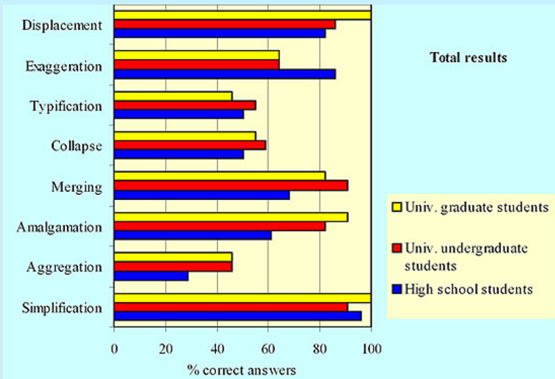
Figure 3: Comparison of the results of the three groups of subjects.
